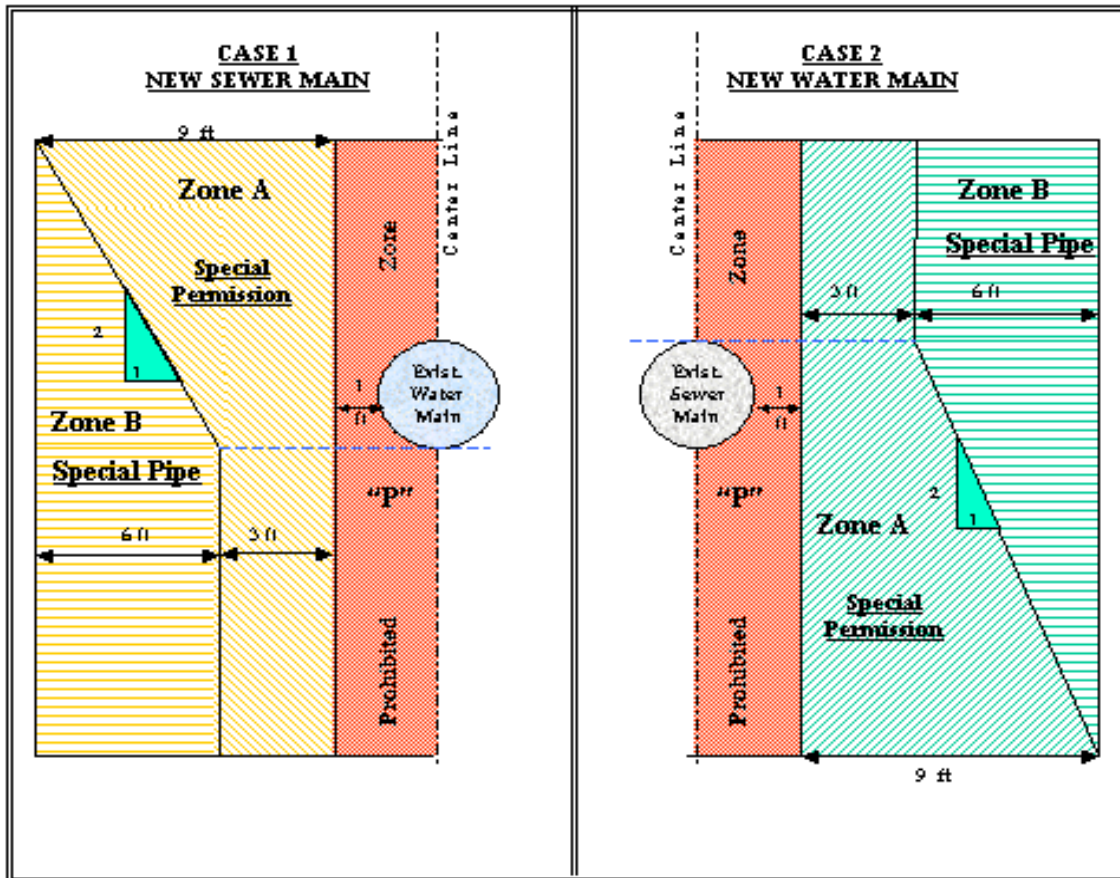
FIGURE 1 PARALLEL CONSTRUCTION
