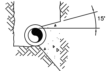
TYPICAL SECTION
