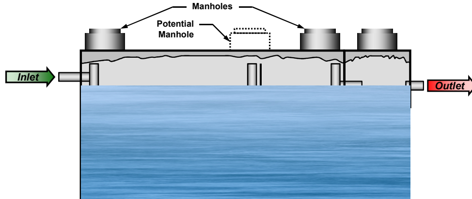
Gravity Grease Interceptor Outdoor, In-ground 500 – 1,500 Gallons (Typical)
