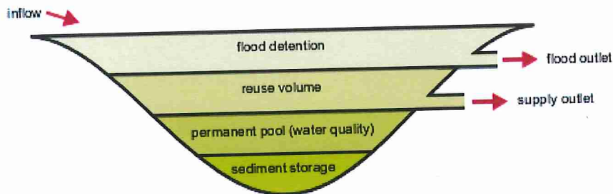
Surface Swale Scheme (NSW Dept. of Environ. & Conservation-2006)
