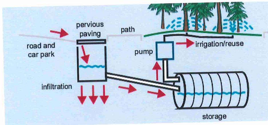
Underground Storage Scheme (NSW Dept. of Environ. & Conservation-2006)
